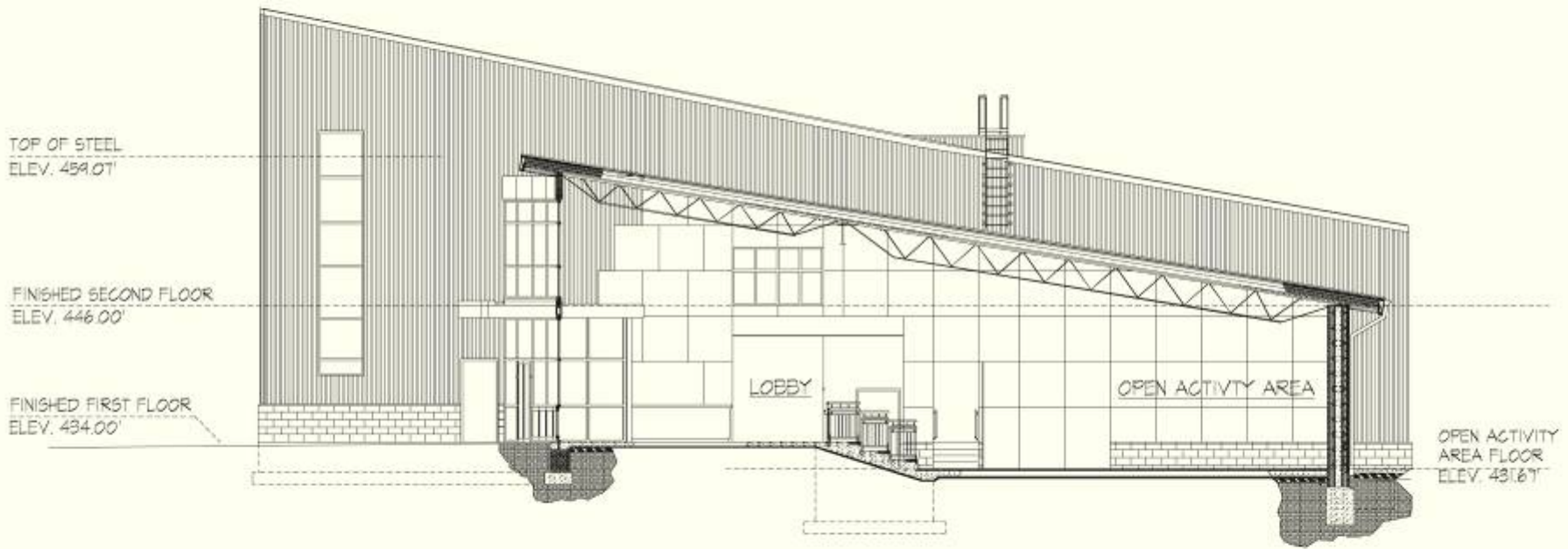
BUILDING SECTION - OPEN ACTIVITY AREA
